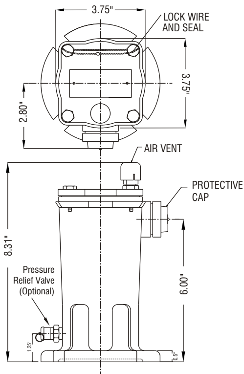
VERTICAL FLANGE MOUNTED
