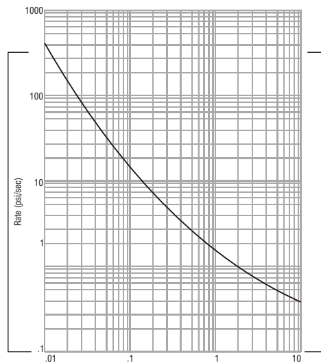
960 Series Response Limits
