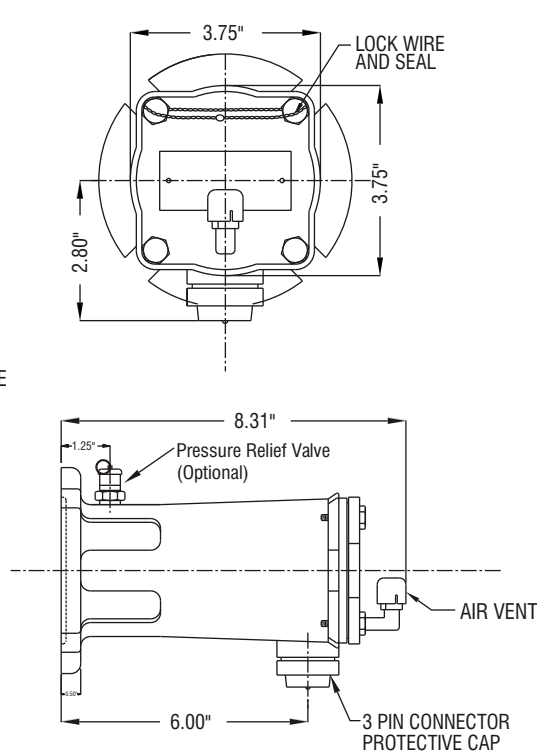
HORIZONTAL FLANGE MOUNTED
